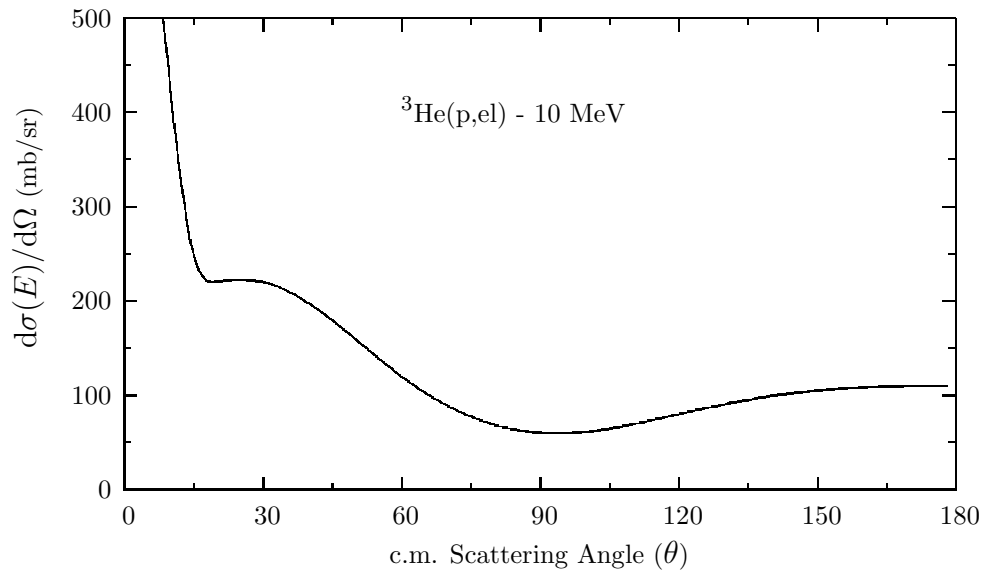
Figure 6.1: Example of Charged-Particle Elastic Scattering Cross Section
